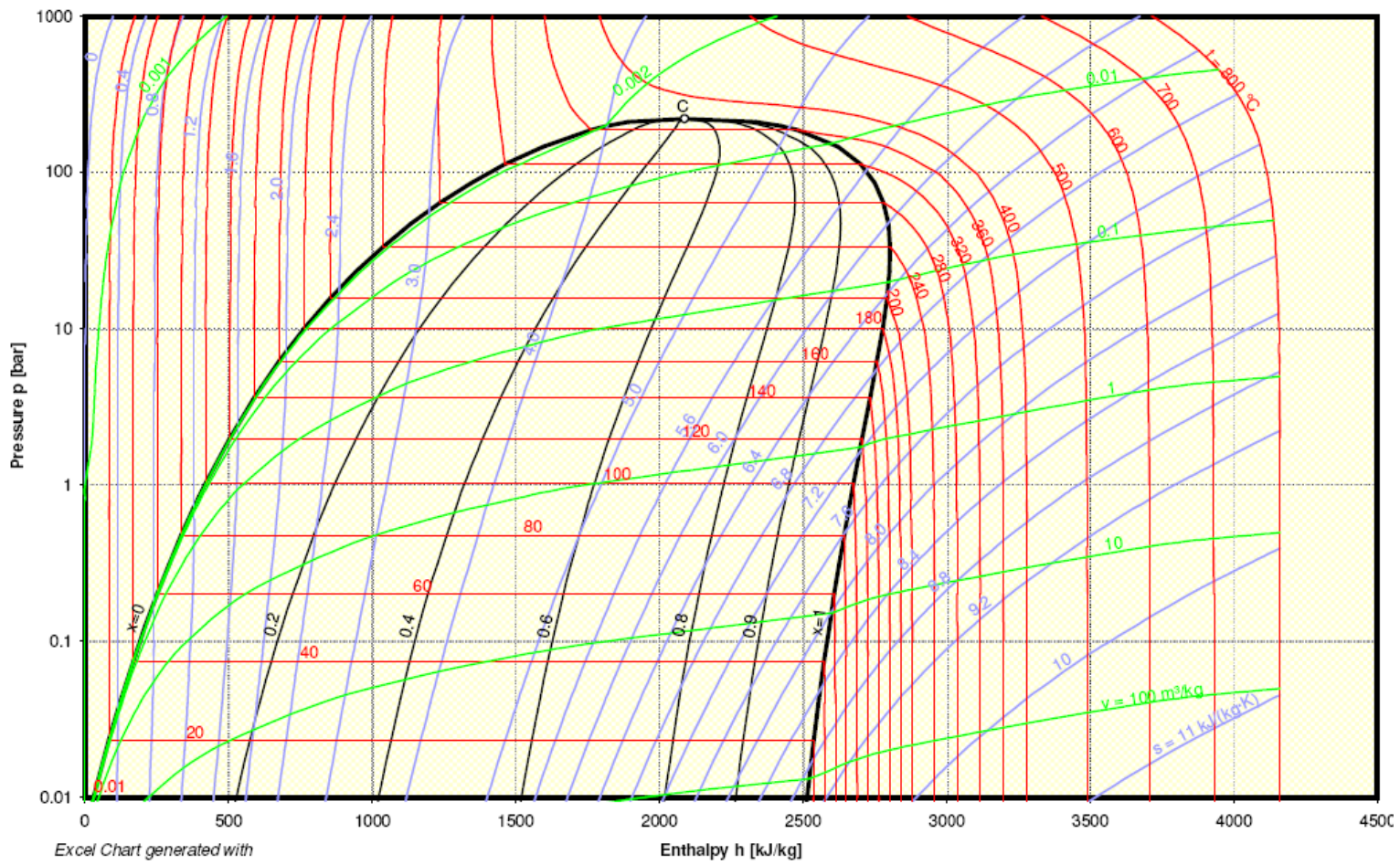
logP-H diagram
