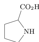
proline
