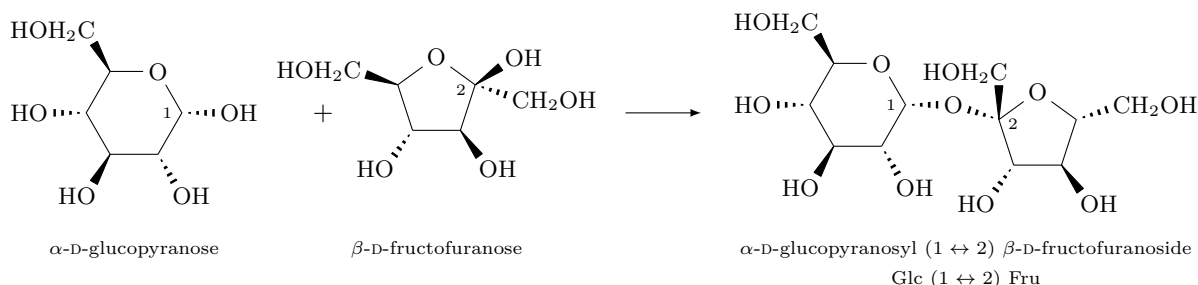
FIGURE 4 – Formation du saccharose.
