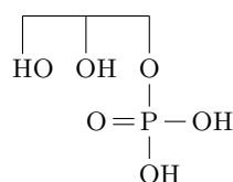
glycérol-3-phosphate
