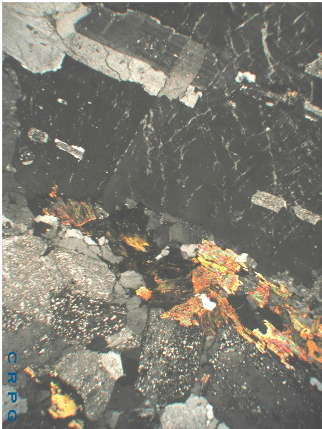
Granite calco-alkalin
