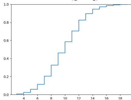
Loi \mathcal{B}(50, \frac{1}{5}) .
