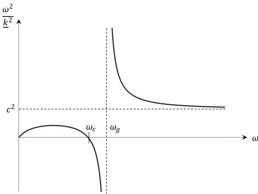
Figure 10 - Relation de dispersion
