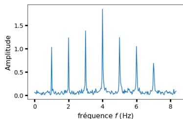
(a) N = 500 ; T_{\max} = 30,0 s
