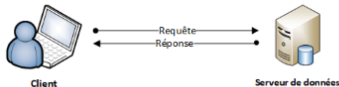
FIGURE 1 – Architecture client-serveur
