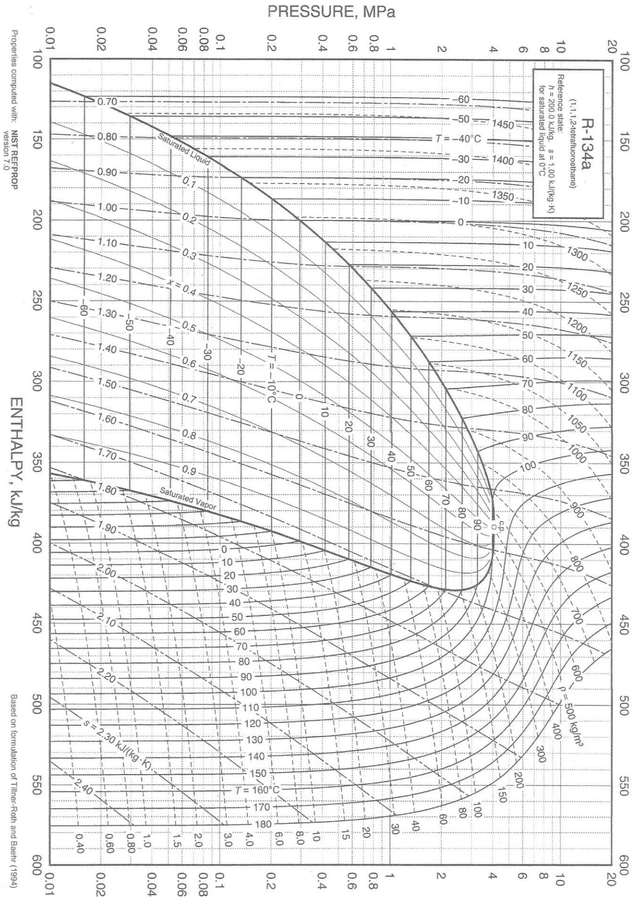
Fig. 8 Pressure-Enthalpy Diagram for Refrigerant R-134a
