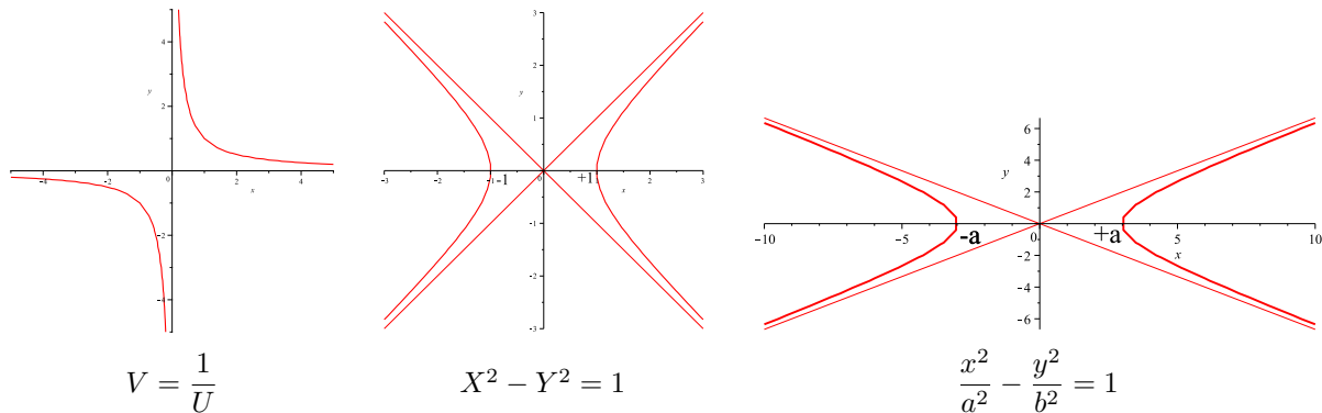
FIGURE XX.2 – HYPERBOLES
