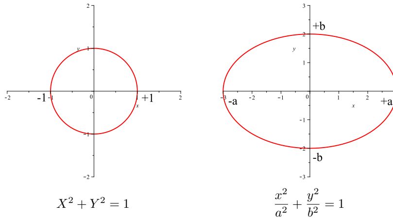
FIGURE XX.1 – CERCLE & ELLIPSE
