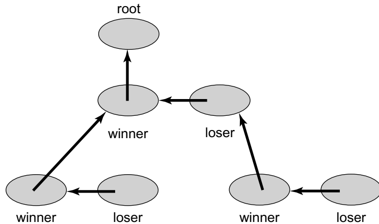
Figure 17.17 The TourBarrier class: information flow. Nodes are paired statically in active/passive pairs. Threads start at the leaves. Each thread in an active node waits for its passive partner to show up; then it proceeds up the tree. Each passive thread waits for its active partner for notification of completion. Once an active thread reaches the root, all threads have arrived, and notifications flow down the tree in the reverse order.
