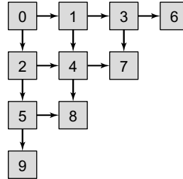
Figure 2.18 Array layout for Bouncer objects.
