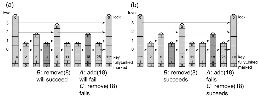
Figure 14.3 The LazySkiplist class: failed and successful add() and remove() calls. In Part (a) the add(18) call finds the node with key 18 unmarked but not yet fully linked. It spins waiting for the node to become fully linked in Part (b), at which point it returns false . In Part (a) the remove(8) call finds the node with key 8 unmarked and fully linked, which means that it can acquire the node's lock in Part (b). It then sets the mark bit, and proceeds to lock the node's predecessors, in this case the node with key 5. Once the predecessor is locked, it physically removes the node from the list by redirecting the bottom-level reference of the node with key 5, completing the successful remove() . In Part (a) a remove(18) fails, because it found the node not fully linked. The same remove(18) call succeeds in Part (b) because it found that the node is fully linked.
