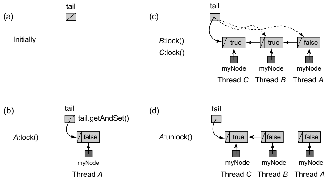
Figure 7.14 A lock acquisition and release in an MCSLock. (a) Initially the tail is null. (b) To acquire the lock, thread A places its own QNode at the tail of the list and since it has no predecessor it enters the critical section. (c) thread B enqueues its own QNode at the tail of the list and modifies its predecessor's QNode to refer back to its own. Thread B then spins on its locked field waiting until A, its predecessor, sets this field from true to false . Thread C repeats this sequence. (d) To release the lock, A follows its next field to its successor B and sets B's locked field to false . It can now reuse its QNode.
