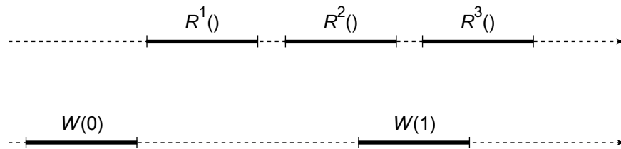
Figure 4.3 A single-reader, single-writer register execution: R^i is the i^{\text{th}} read and W(v) is a write of value v . Time flows from left to right. No matter whether the register is safe , regular , or atomic , R^1 must return 0, the most recently written value. If the register is safe then because R^2 and R^3 are concurrent with W(1) , they can return any value in the range of the register. If the register is regular , R^2 and R^3 can each return either 0 or 1. If the register is atomic then if R^2 returns 1 then R^3 also returns 1, and if R^2 returns 0 then R^3 could return 0 or 1.
