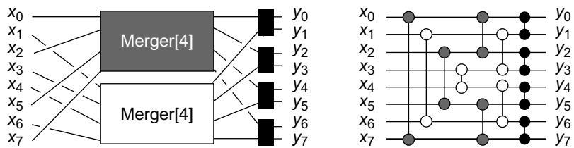
Figure 12.12 On the left-hand side we see the logical structure of a \text{MERGER}[8] network, into which feed two \text{BITONIC}[4] networks, as depicted in Fig. 12.12. The gray \text{MERGER}[4] network has as inputs the odd wires coming out of the top \text{BITONIC}[4] network, and the even ones from the lower \text{BITONIC}[4] network. In the lower \text{MERGER}[4] the situation is reversed. Once the wires exit the two \text{MERGER}[4] networks, each pair of identically numbered wires is combined by a balancer. On the right-hand side we see the physical layout of a \text{MERGER}[8] network. The different balancers are color coded to match the logical structure in the left-hand figure.
