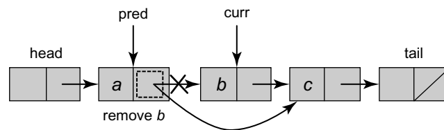
Figure 9.3 A sequential Set implementation: adding and removing nodes. In Part (a), a thread adding a node b uses two variables: curr is the current node, and pred is its predecessor. The thread moves down the list comparing the keys for curr and b . If a match is found, the item is already present, so it returns false. If curr reaches a node with a higher key, the item is not in the set so Set b 's next field to curr , and pred 's next field to b . In Part (b), to delete curr , the thread sets pred 's next field to curr 's next field.
