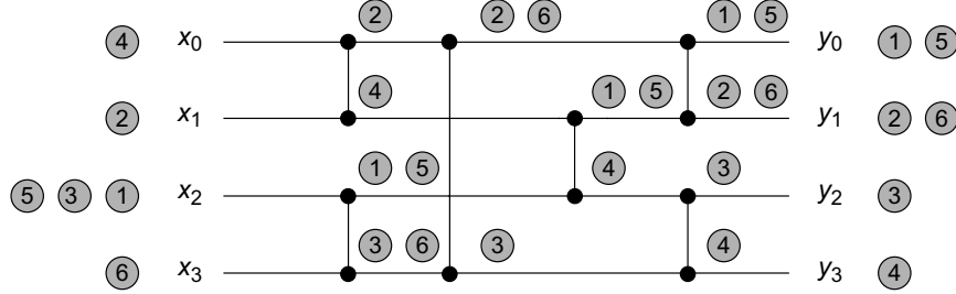
Figure 12.11 A sequential execution of a BITONIC [4] counting network. Each vertical line represents a balancer, and each balancer's two input and output wires are the horizontal lines it connects to at the dots. In this sequential execution, tokens pass through the network, one completely after the other in the order specified by the numbers on the tokens. We track every token as it passes through the balancers on the way to an output wire. For example, token number 3 enters on wire 2, goes down to wire 1, and ends up on wire 3. Notice how the step property is maintained in every balancer, and also in the network as a whole.
