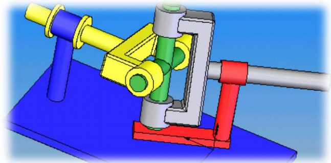
joint de cardan simple
