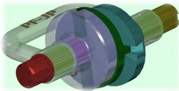
joint de Oldham
