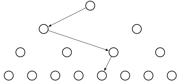
FIGURE 11 – Programmation gloutonne
