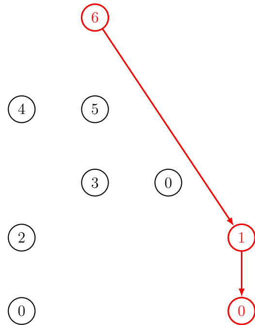
FIGURE 7 – Rendu glouton
