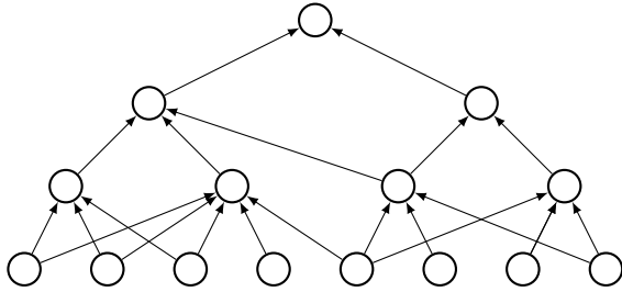
FIGURE 10 – Programmation dynamique
