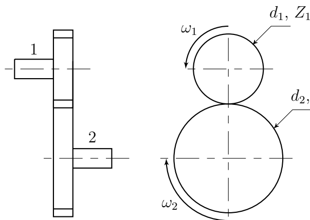
FIGURE 4 – Engrenages parallèles.
