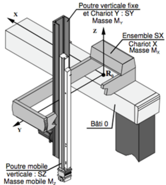
FIGURE 4.2 – Sous-ensembles mobiles.
