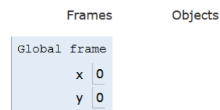
FIGURE 1. – variable non mutable x
