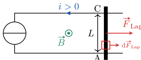
FIGURE I2.3 – Schéma rails.
