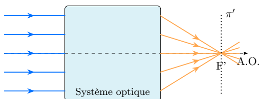
FIGURE O2.20 – Foyer principal image.
