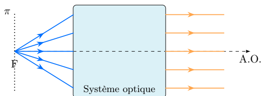
FIGURE O2.19 – Foyer principal objet.
