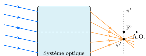
FIGURE O2.22 – Foyer secondaire image.
