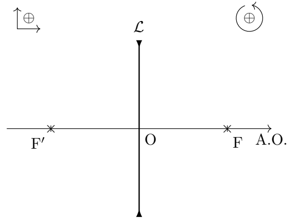
FIGURE O3.7 – Foyer image divergent
