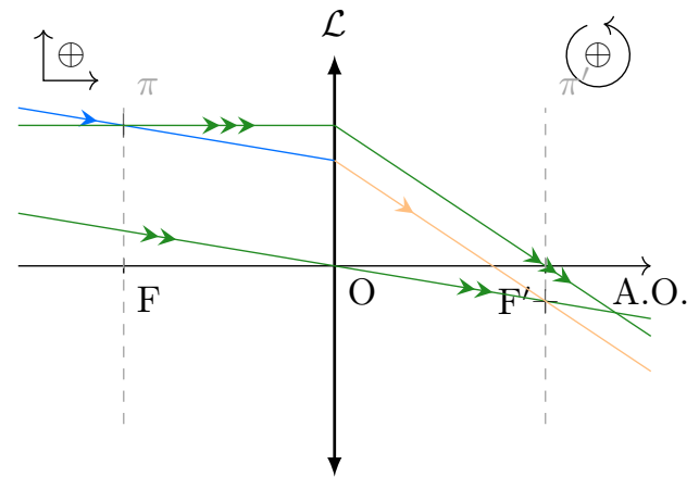
FIGURE O3.6 – f – Convergente rayon quelconque
