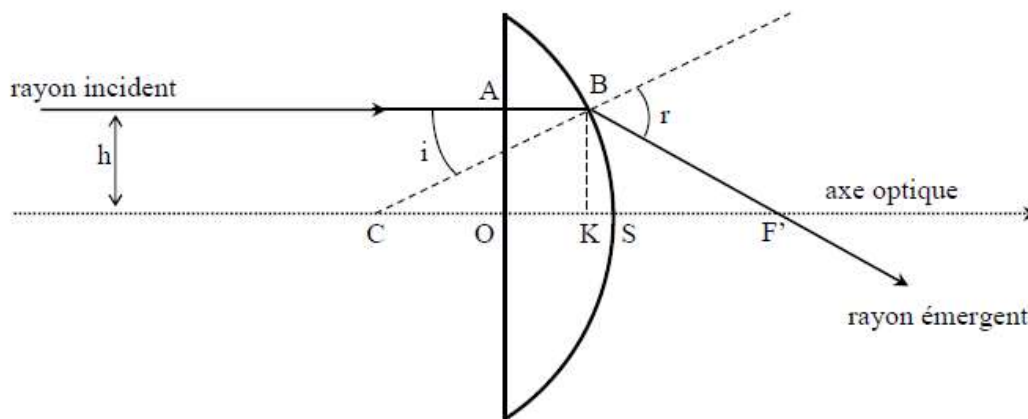
FIGURE 9 – Lentille plan-convexe.
