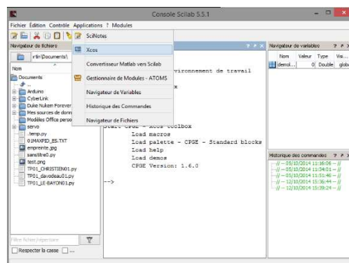
Figure 4 : Lancer Xcos
