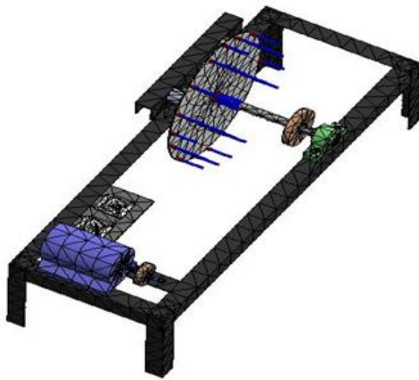
Fig 5.2 (Stress Distribution on CAD Model)
