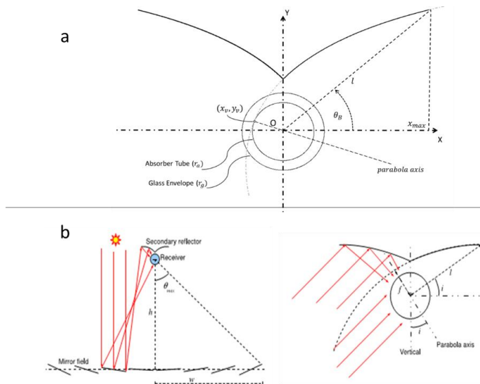
Fig. 6. Vacuum tubular absorber with butterfly secondary concentrator: a) [41] b) [33]
