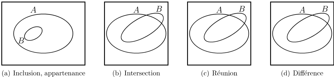
FIGURE 1.1 – Diagrammes de Venn
