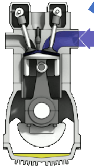
Soupape (SolidWorks)
