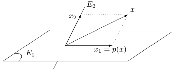
FIGURE 1 – E = E_1 \oplus E_2
