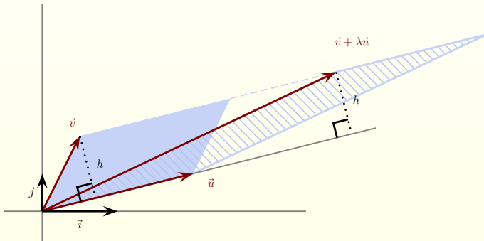
Figure 2 - \mathcal{A}(\mathcal{P}_{\vec{u}, \vec{v} + \lambda \vec{u}}) = \mathcal{A}(\mathcal{P}_{\vec{u}, \vec{v}}) .
